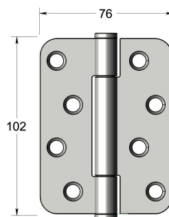
Dimensions drawing (DIM)
