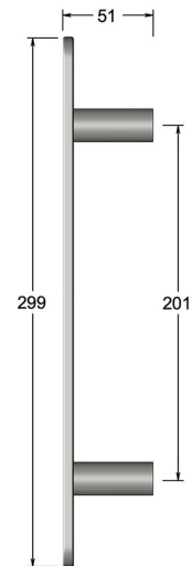
Dimensions drawing (DIM)
