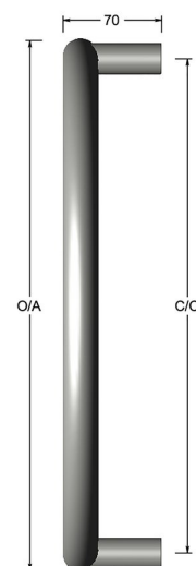
Dimensions drawing (DIM)
