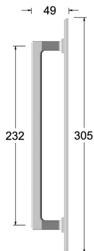
Dimensions drawing (DIM)
