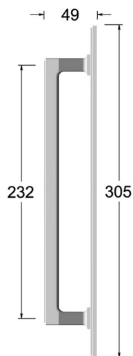
Dimensions drawing (DIM)
