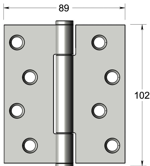
Dimensions drawing (DIM)
