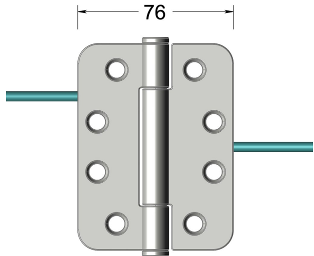
Dimensions drawing (DIM)
