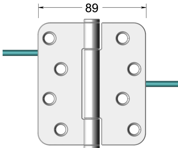
Dimensions drawing (DIM)
