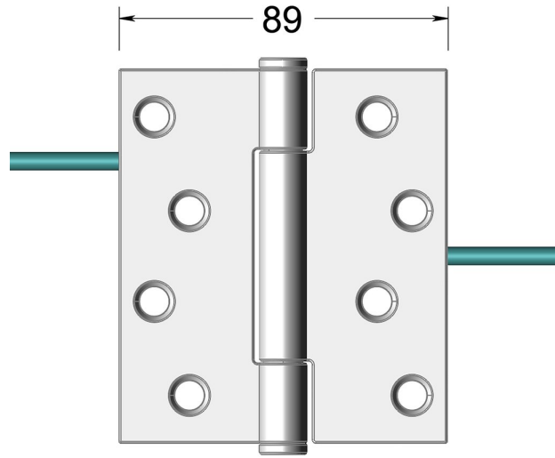
Dimensions drawing (DIM)
