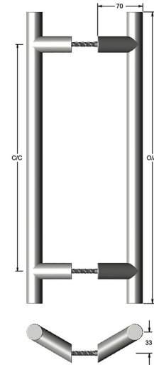
Dimensions drawing (DIM)
