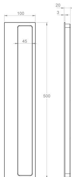
Dimensions drawing (DIM)
