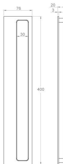
Dimensions drawing (DIM)
