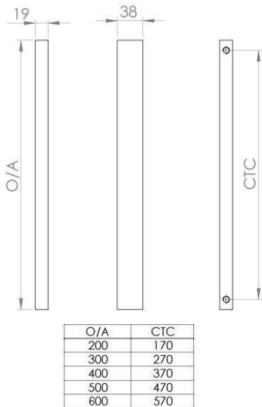
Dimensions drawing (DIM)
