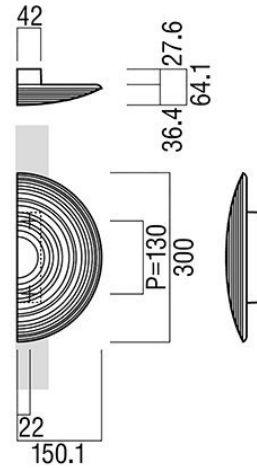
Dimensions drawing (DIM)
