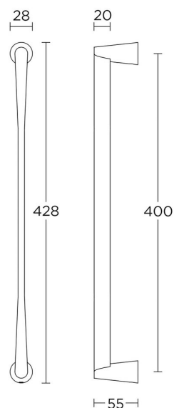
Dimensions drawing (DIM)
